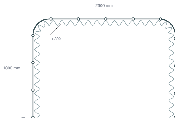
PLAN · fixing points at ≤500 mm centres · Wave 80 curtain shown
