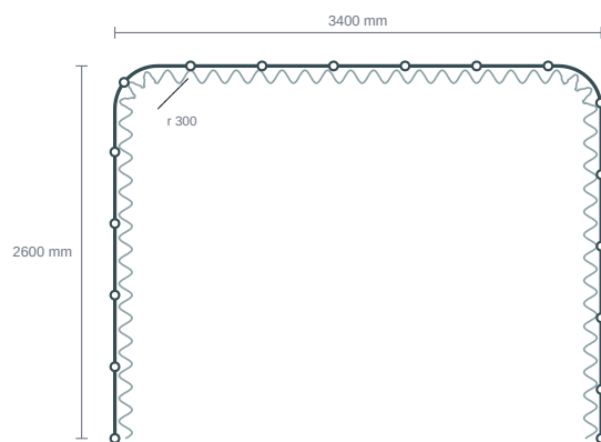
PLAN · fixing points at ≤500 mm centres · Wave 80 curtain shown
