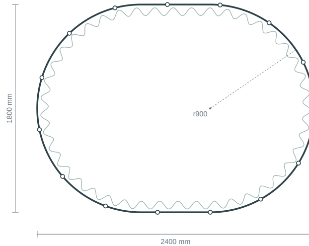
PLAN · fixing points at ≤500 mm centres · Wave 80 curtain shown
