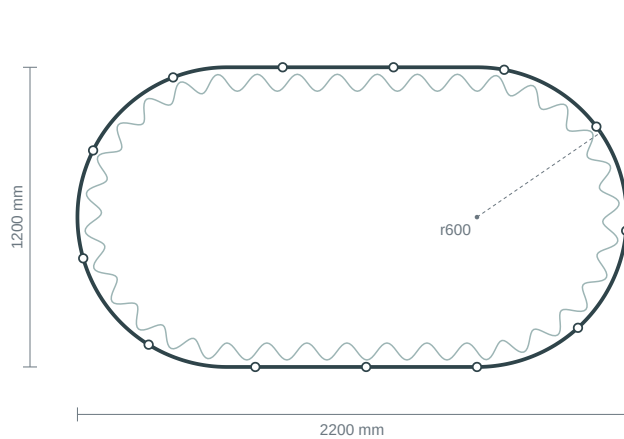
PLAN · fixing points at ≤500 mm centres · Wave 80 curtain shown
